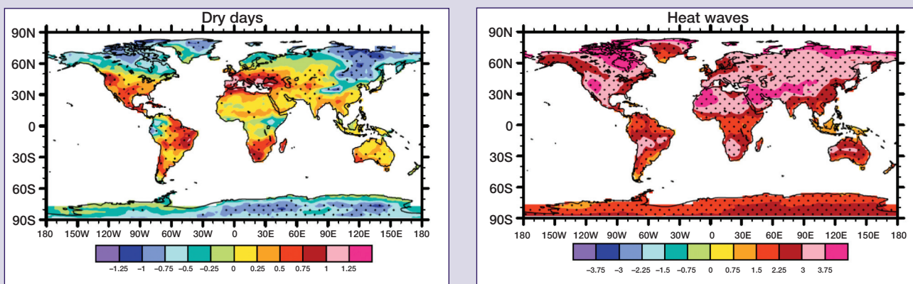
WebFigure 1. Examples of predicted global changes in dry days and heat waves from the late 20th century to the late 21st century under IPCC scenario A1B (from Tebaldi et al. 2006). The “dry days” index is defined as the maximum number of consecutive dry days in a year, and “heat waves” are the maximum periods of at least five consecutive days with maximum temperature at least 5 °C higher than the 1961–1990 mean for the same calendar day. Values are changes in multi-model averages in standardized units. Stippled regions show where five of the nine models used in the analysis predict statistically significant changes. Tebaldi et al. (2006) found general trends toward increasing extremes of ten indicators of temperature and extreme precipitation events, but with substantial regional variability and differences among models. The coarse resolution of available global models (varying in these nine from 1–5 °C resolution) also suggests that there is more local heterogeneity than depicted by these maps. With kind permission from Springer Science and Business Media.
